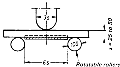
Figure 15. Welding bend test
